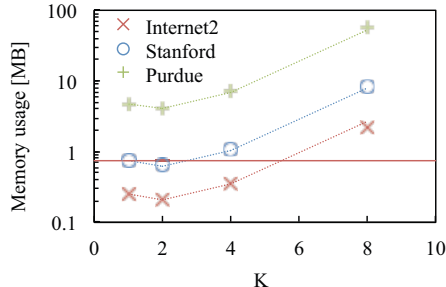
Fig. 6. Memory usage of MDD. The dotted lines indicate (10). The horizontal line is memory usage of HybridCuts for Internet2.
