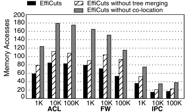
FIGURE 10. Impact of Tree Merging & Co-location
